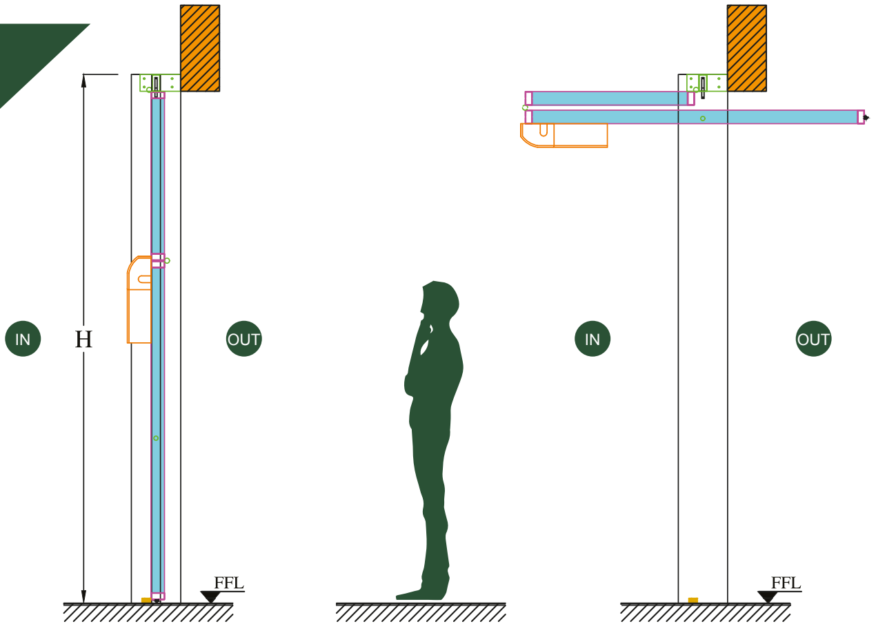
Side View (Closed)
