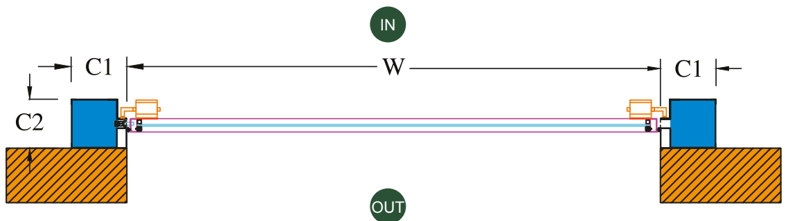
Top View
