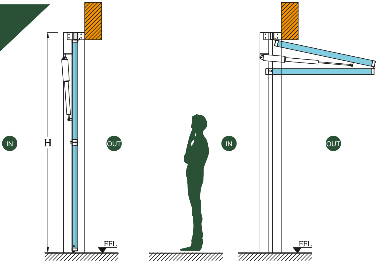
Side View (Closed)
