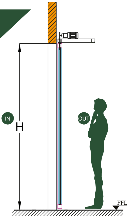
Side View (Closed)
