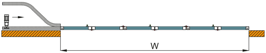
Top View (Closed)
