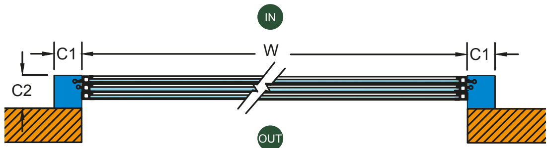
Top View
